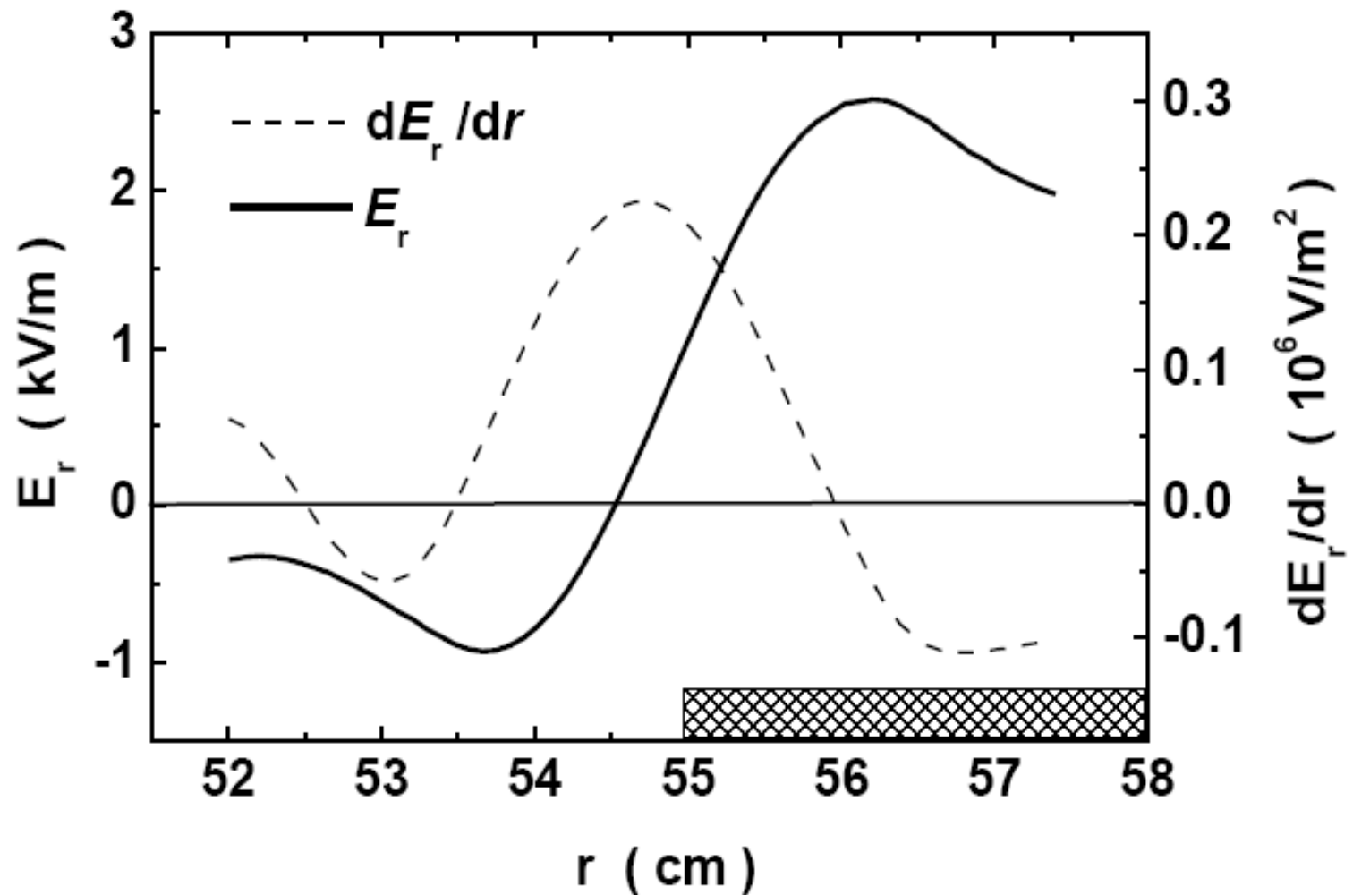
Fig. 4 Radial profiles of radial electric field E_r (estimated from the fit curve of the plasma potential) and its radial gradient dE_r/dr . It can be seen that a naturally formed poloidal velocity shear layer (VSL) is located near the radial position of the limiter.
