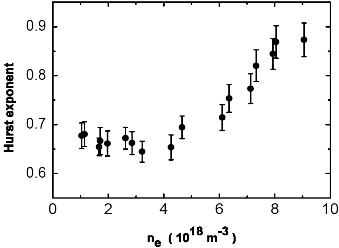
Fig. 9 Profile of the Hurst exponents, H , versus the electron density. The Hurst exponent, an indication of the long-range time correlations of the flux time series, is evaluated from the R/S statistics. We can see that at all measured positions the values of H are larger than 0.5, i.e. there exist long-range time dependencies in the turbulent transport in SUNIST edge. Furthermore, as the density increases, the values of H are greater than 0.8, indicating a stronger long-range time dependencies.
