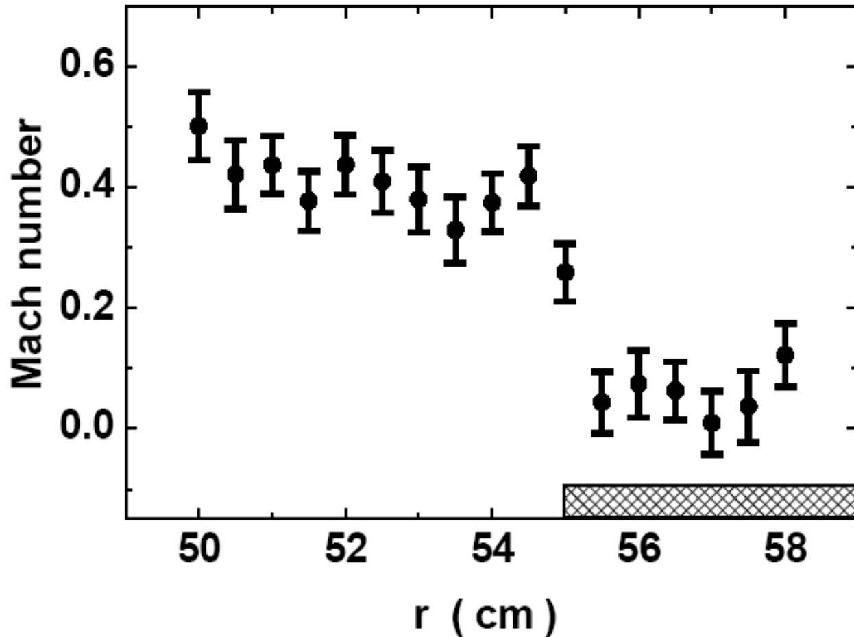
Fig. 5 Radial profile of the toroidal flow velocity Mach number M . In SOL, M \sim 0.1 and the toroidal velocity v_\phi \sim 3.4 \text{ km s}^{-1} ; but in the plasma edge, M \sim 0.4 and v_\phi \sim 13 \text{ km s}^{-1} . A maximal radial gradient of the v_\phi appears at the radial location of the VSL. Such coincidence was first observed on the TEXT-U tokamak, but it seems not to be reported on the spherical tokamaks so far.
