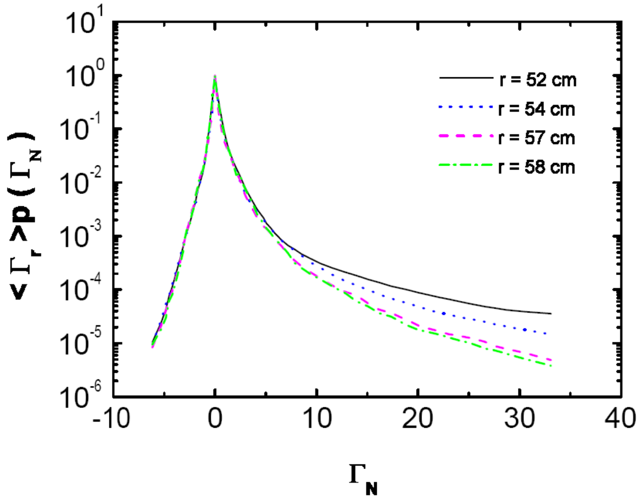
Fig. 11 Comparison of the normalized PDF of the fluxes measured in four different radial positions. We can see that all four PDFs have a clear non-Gaussian long time lag tails, which are the signature of long-range correlation transport events. Furthermore, the PDFs in high-density case (at plasma edge) have a little larger tails than that in low-density case (at SOL).
