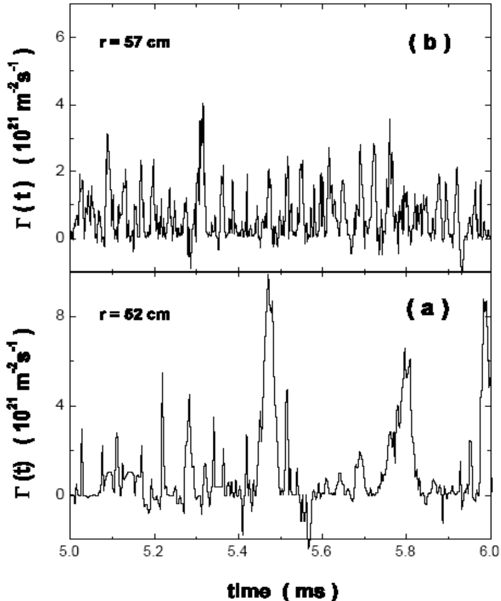
Fig. 7 Comparison of the particle flux patterns between the data from SOL and that from plasma edge.
