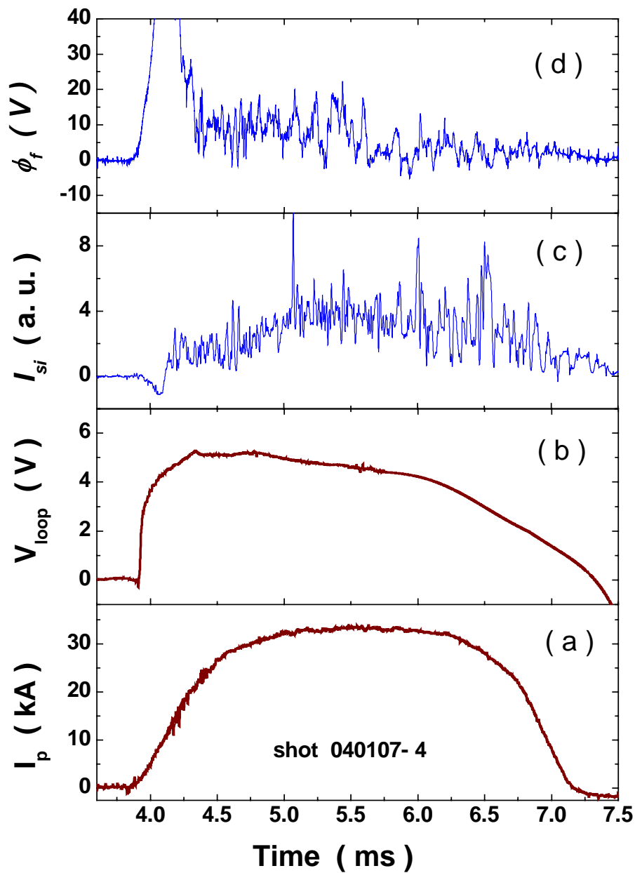
Fig. 2 Typical discharge waveforms of (a) the plasma current, (b) loop voltage, (c) ion saturation current and (d) floating potential.
