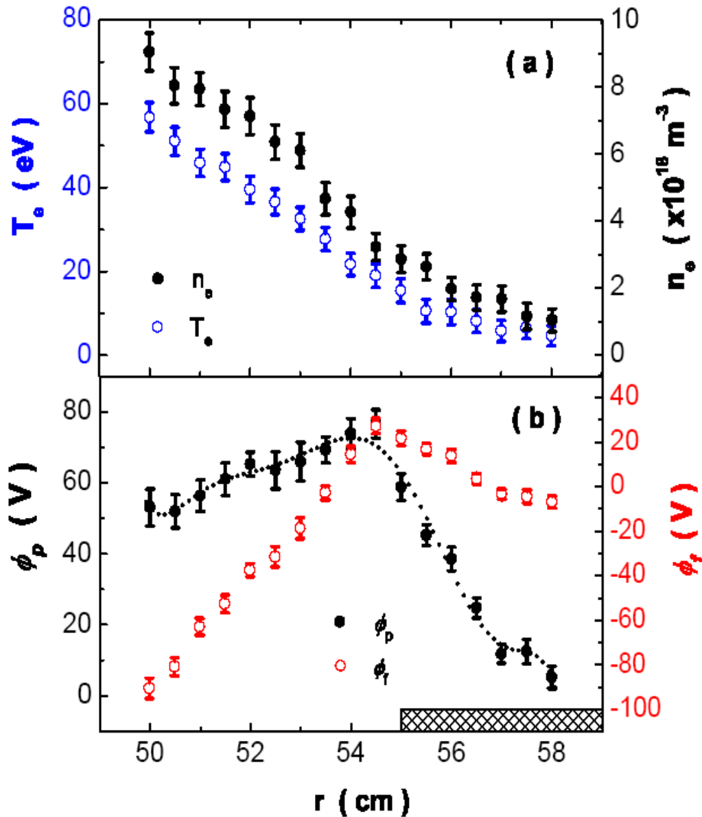
Fig. 3 Radial profiles of equilibrium T_e , n_e , \phi_f and \phi_p
