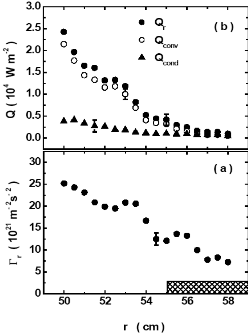
Fig. 6 Radial profiles of (a) the radially turbulence-induced particle fluxes \Gamma_r , and (b) the heat fluxes Q_r , Q_{\text{conv}} and Q_{\text{cond}} . Here
