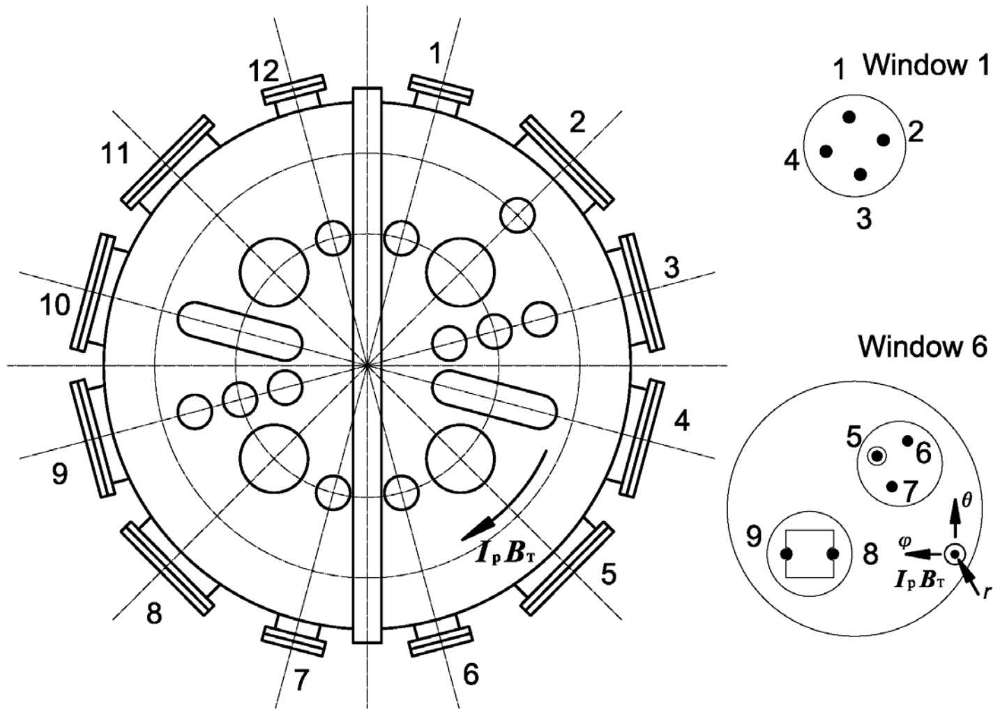
Fig. 1 Relative positions of the windows where the probe arrays are laid, and a closed-up view of the probe structures.
