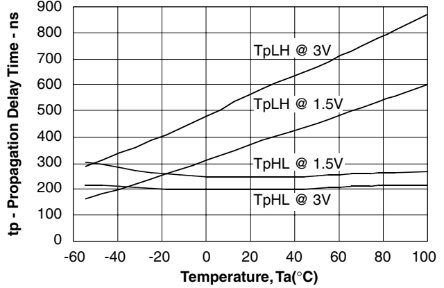
Figure 9. Propagation Delay vs. Temperature-6N135 @ V_{CC}=5.0\text{ V} , I_F=16\text{ mA} , R_L=4.1\text{ k}\Omega
