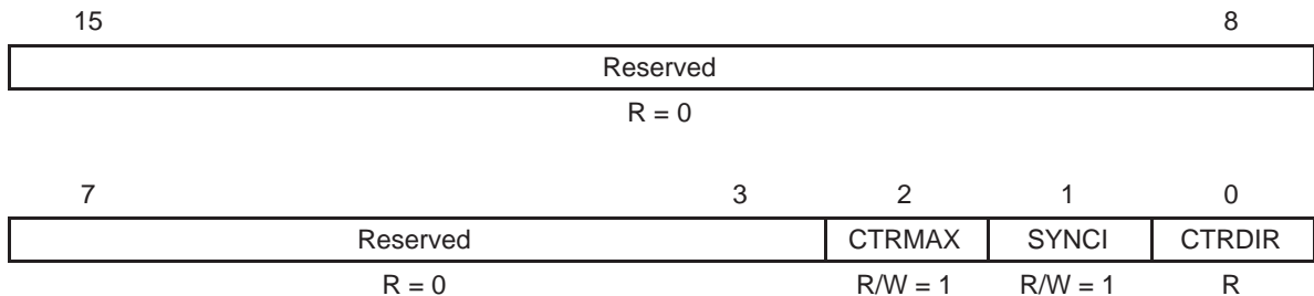
Figure 4–5. TB Status Register (TBSTS)
