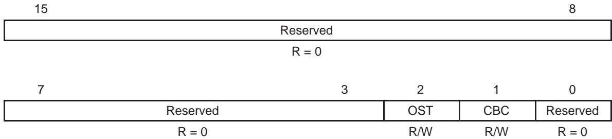
Figure 4–19. TZ Enable Interrupt Register (TZEINT)
