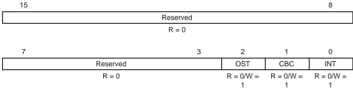
Figure 4–21. TZ Clear Register (TZCLR)
