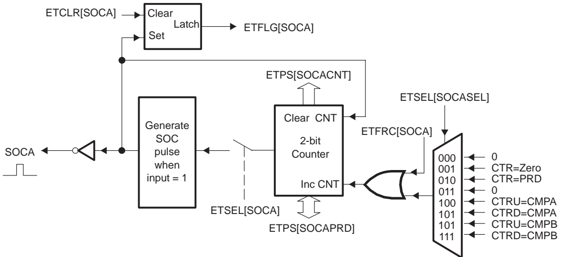
Figure 2–38. ET Register Bits Interacting with ET SOCA Pulse Generator
