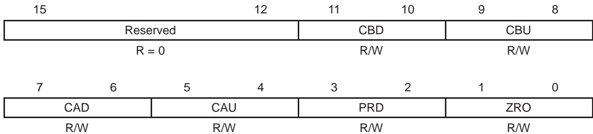
Figure 4–10. AQ Output B Control Register (AQCTLB)
