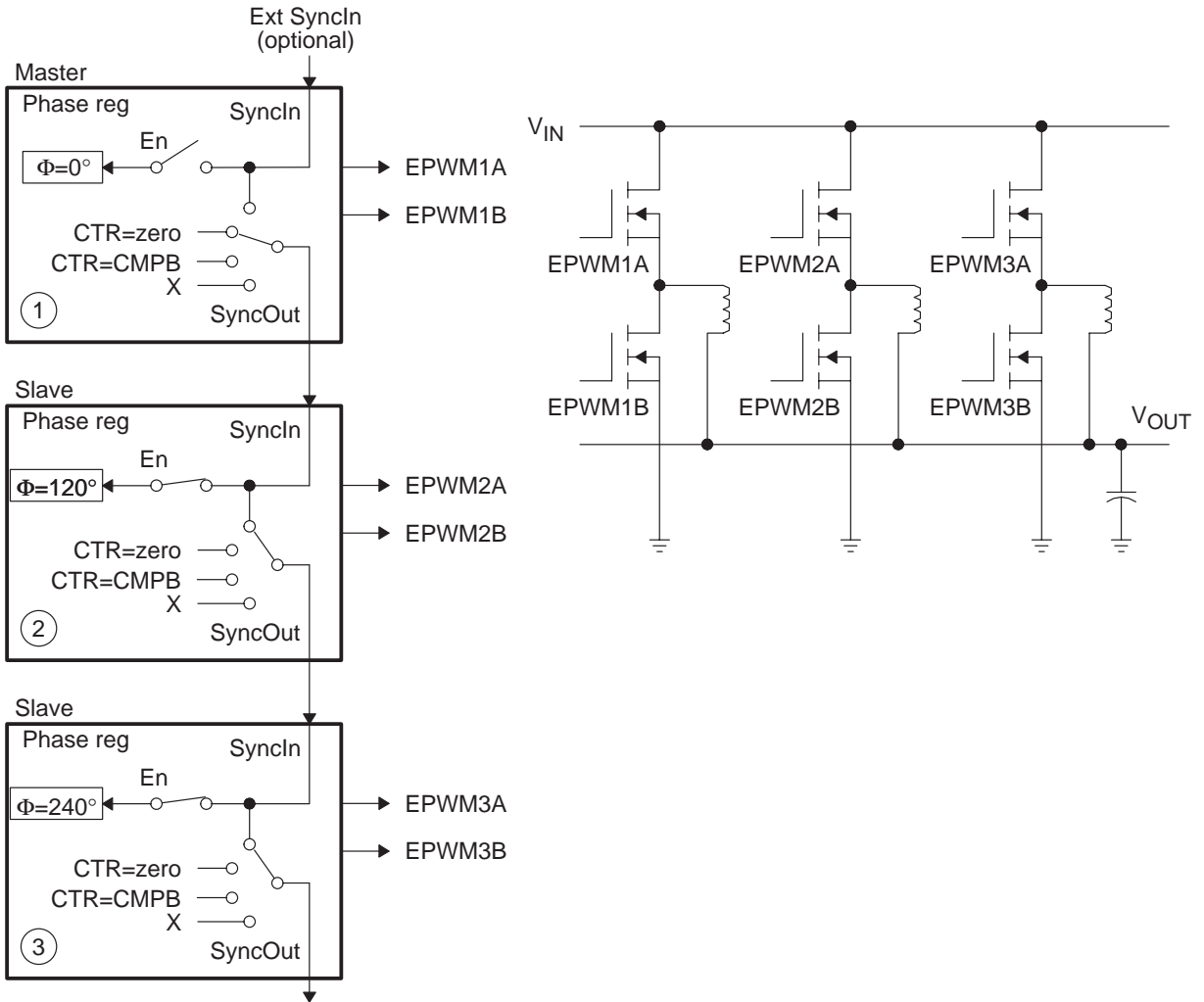
Figure 3-14. Control of a 3-Phase Interleaved DC/DC Converter
