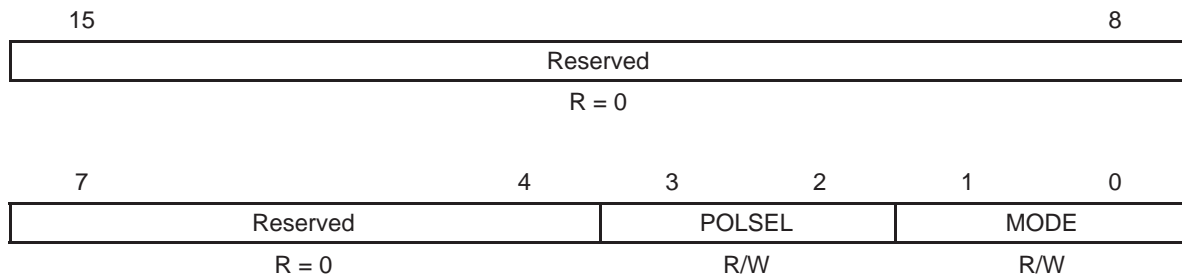
Figure 4–13. DB Generator Control Register (DBCTL)
