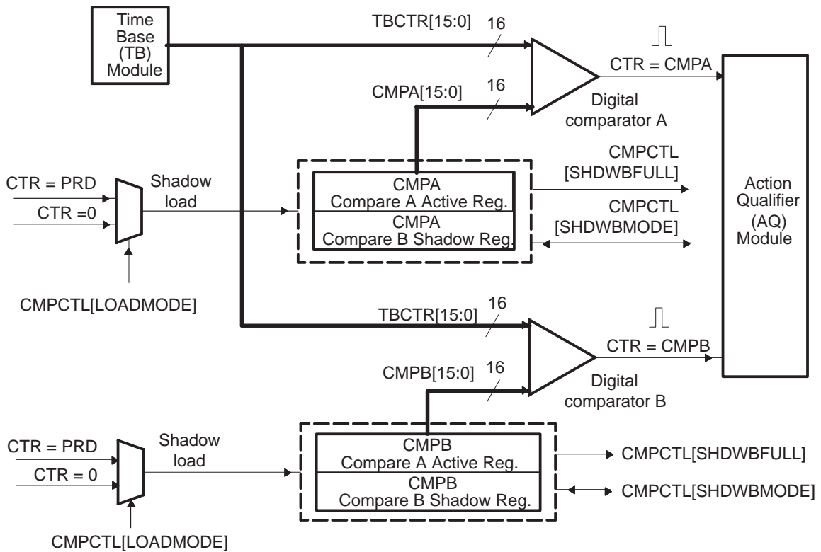
Figure 2–9. Detailed View of the CC Module
