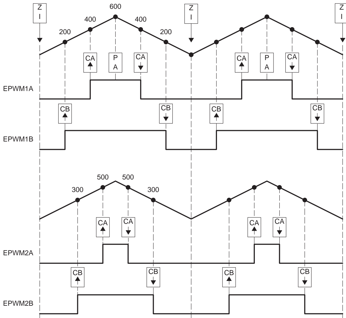
Figure 3-6. Buck Waveforms for Figure 3-5 (Note: F_{PWM2} = F_{PWM1} )
