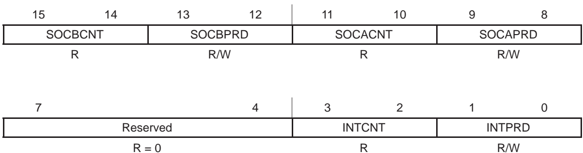
Figure 4–24. ET Prescale Register (ETPS)
