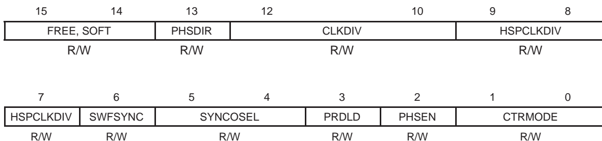
Figure 4–4. TB Control Register (TBCTL)
