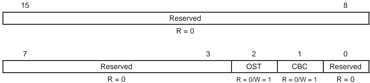
Figure 4–22. TZ Force Register (TZFRC)
