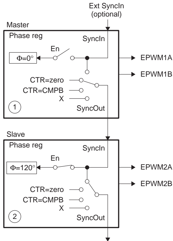
Figure 3–12. Configuring Two PWM Modules for Phase Control
