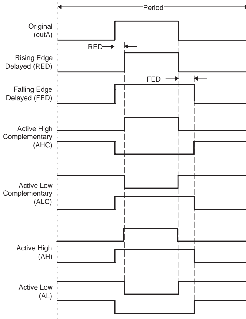
Figure 2–25. DB Module Waveforms for Typical Cases ( 0\% < \text{Duty} < 100\% )
