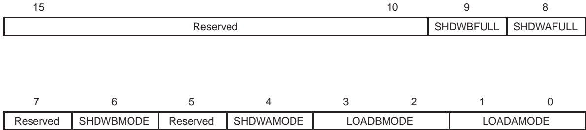
Figure 4–8. Compare Control Register (CMPCTL)
